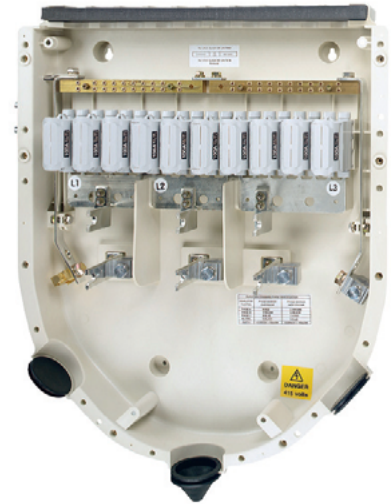
MSDB 10 way fused incomer
