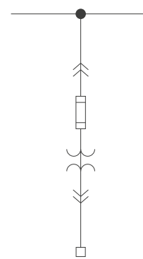
Disconnecter function
